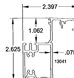
29 BOTTOM SASH BOTTOM RAIL
