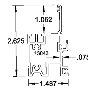
14 TOP SASH BOTTOM RAIL
