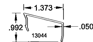
5 HEAD SCREW COVER
