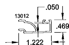
16 BEADING 7/16
