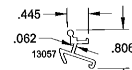
31 BOTTOM LOCK
